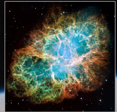
CRAB NEBULA
